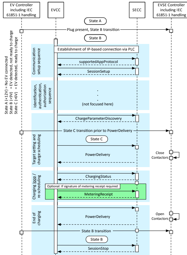
Figure 1: AC request-response message sequence with PnC
